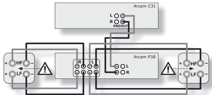
A P35 connected to speakers using bi-wiring.
