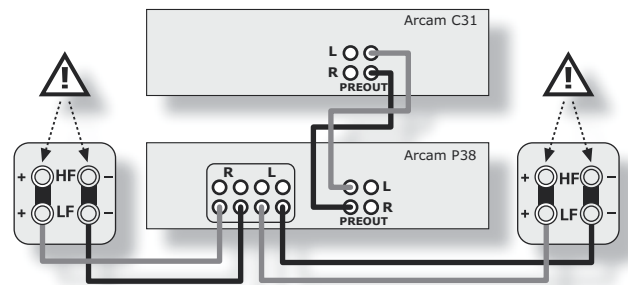
A P35 connected to speakers using single wiring.
