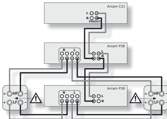
A P35 connected to speakers using bi-amping.
